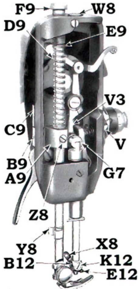
FIG. 52. TO REMOVE NEEDLE BAR AND PRESSER BAR
