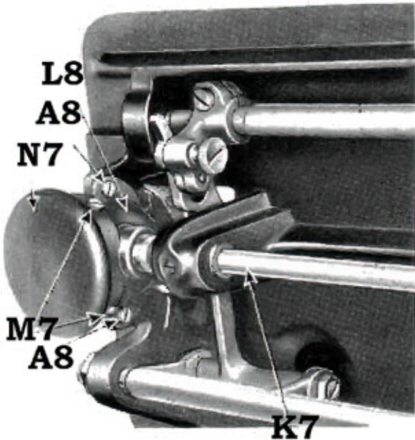
FIG. 34. REMOVING ROTATING HOOK SHAFT BEVEL GEAR COVER
