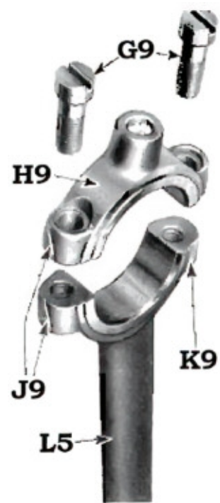
FIG. 54. FEED CONNECTING ROD REMOVED SHOWING UPPER END
