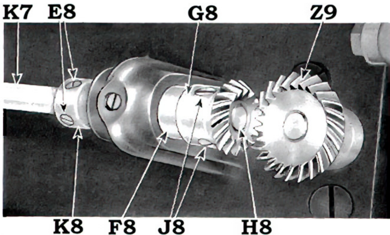
FIG. 39. TO REMOVE ROTATING HOOK DRIVING SHAFT AND ROTATING HOOK DRIVING SHAFT BACK BEVEL GEAR
