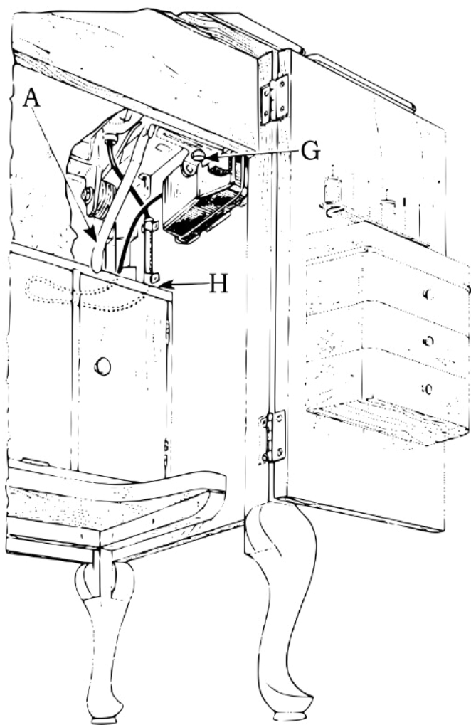
FIG. 6. BAKELITE CONTROLLER ARRANGED FOR KNEE CONTROL IN CABINET 48
