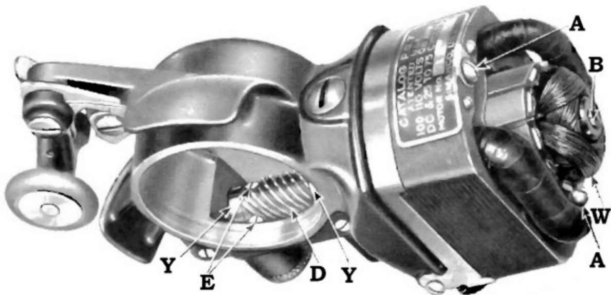
FIG. 16. MOTOR WITH COVER REMOVED MACHINE 201-2 (ARMATURE PARTLY REMOVED)
