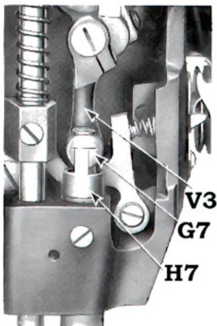
FIG. 32. CORRECT ADJUSTMENT OF TIMING GAUGE
