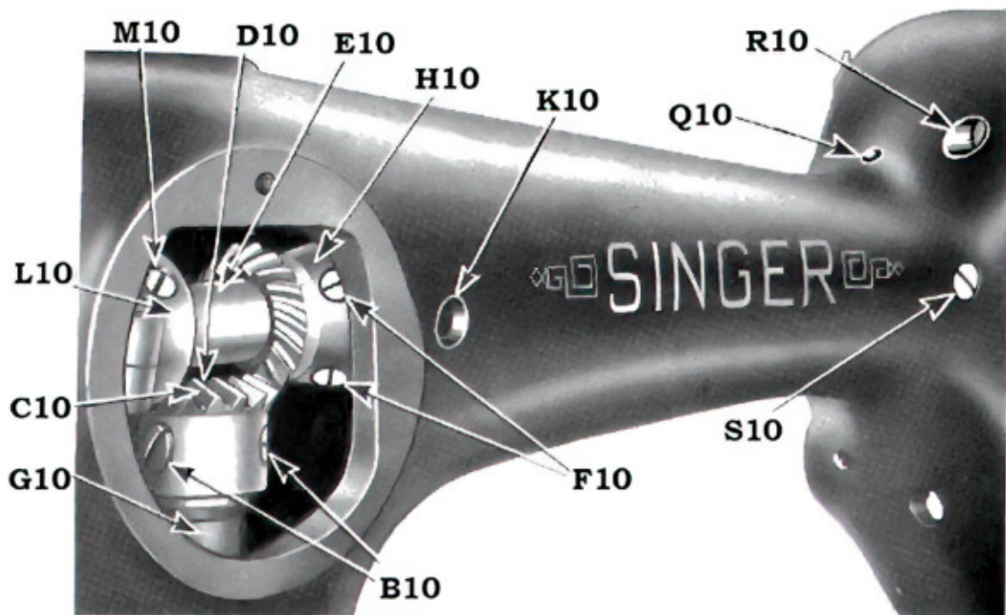
FIG. 59. TO REMOVE HORIZONTAL ARM SHAFT (VIEW THROUGH ARM SIDE COVER OPENING)
