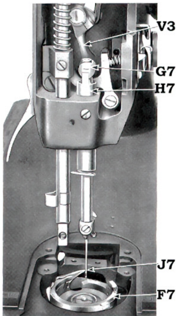
FIG. 33. NEEDLE BAR AND ROTATING HOOK CORRECTLY TIMED
