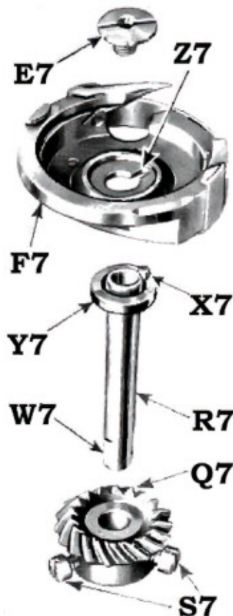
FIG. 37. ROTATING HOOK SHAFT AND GEAR (REMOVED AND DISASSEMBLED)
