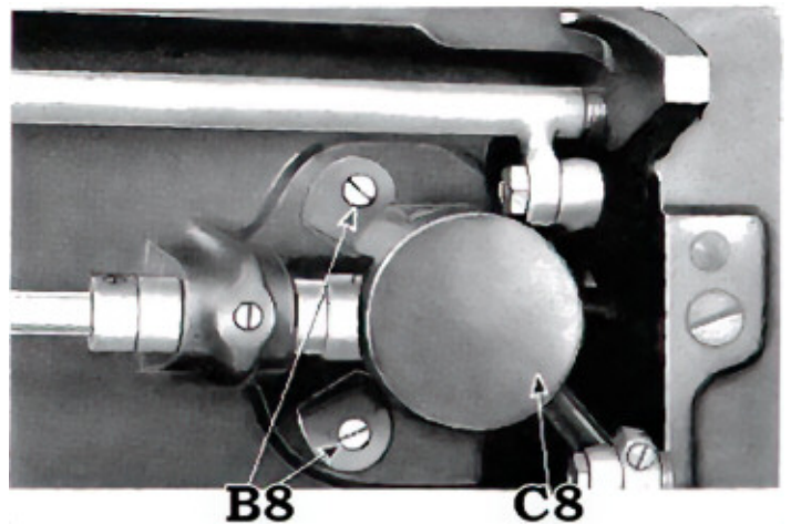
FIG. 38. REMOVING ROTATING HOOK DRIVING SHAFT BEVEL GEAR BACK COVER
