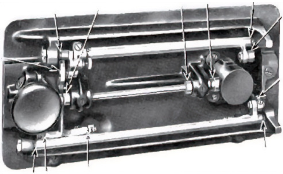
FIG. 67. OILING POINTS IN BASE OF MACHINE
