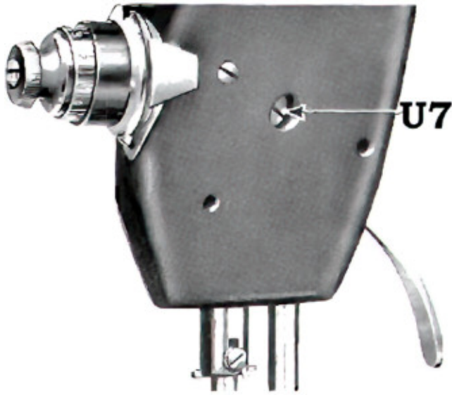
FIG. 36. SCREW TO ADJUST NEEDLE BAR HEIGHT
