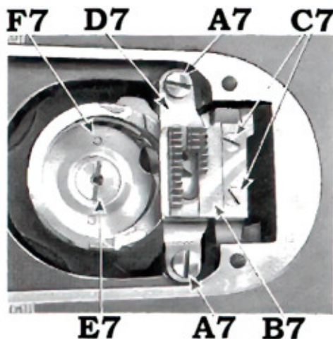
FIG. 31. TO REMOVE ROTATING HOOK
