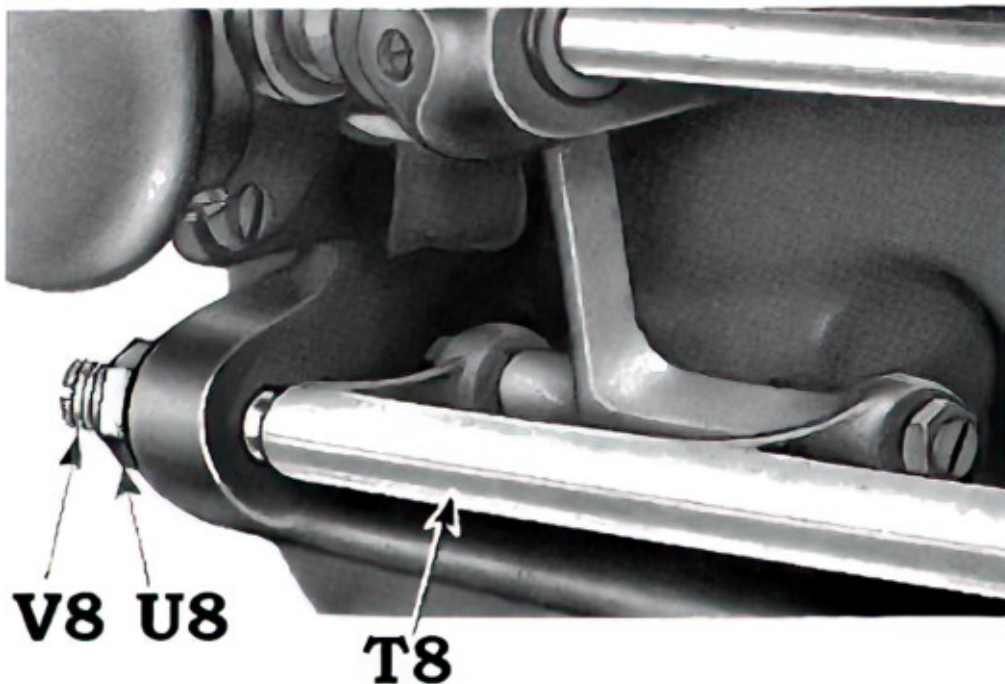
FIG. 42. SIDEWISE ADJUSTMENT OF FEED DOG
