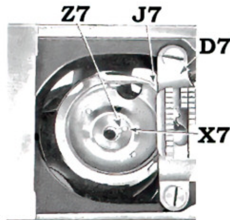
FIG. 31A. TO REMOVE ROTATING HOOK
