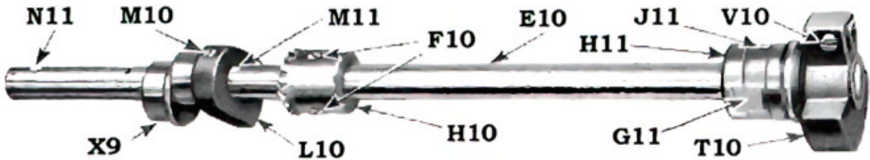
FIG. 62. HORIZONTAL ARM SHAFT REMOVED SHOWING THE POSITIONS OF NEEDLE BAR CRANK, BUSHING, GEAR AND ECCENTRICS ON THE SHAFT
