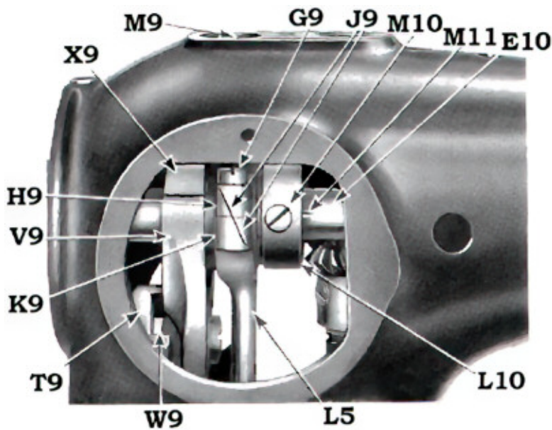
FIG. 53. TO REMOVE FEED CONNECTING ROD
