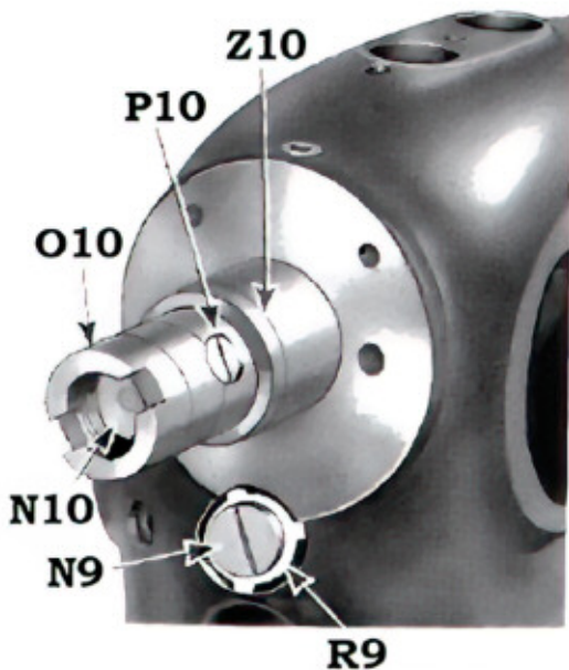
FIG. 56. TO REMOVE FEED REGULATOR
