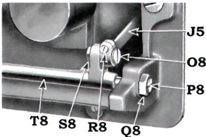
FIG. 41. LENGTHWISE ADJUSTMENT OF FEED DOG
