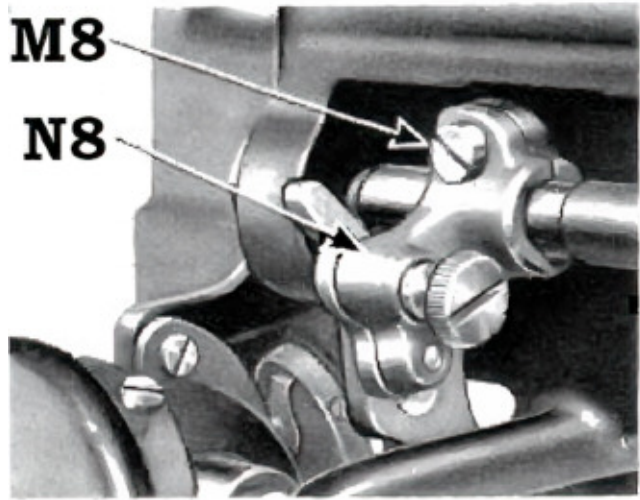
FIG. 40. TO RAISE OR LOWER THE FEED DOG
