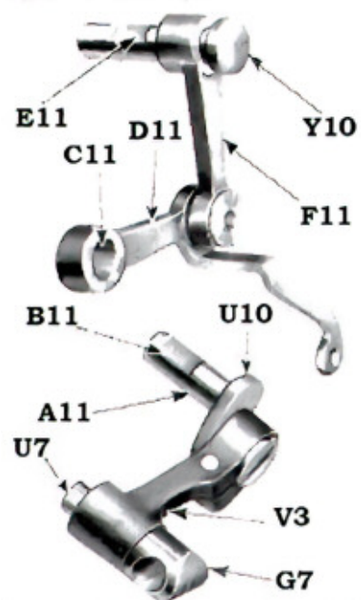
FIG. 61. THREAD TAKE-UP LEVER ASSEMBLY AND NEEDLE BAR LINK REMOVED FROM MACHINE
