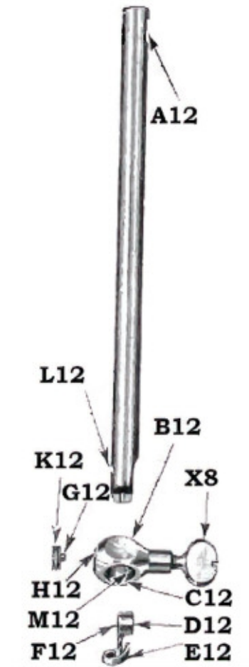
FIG. 52A. NEEDLE BAR REMOVED AND DISASSEMBLED
