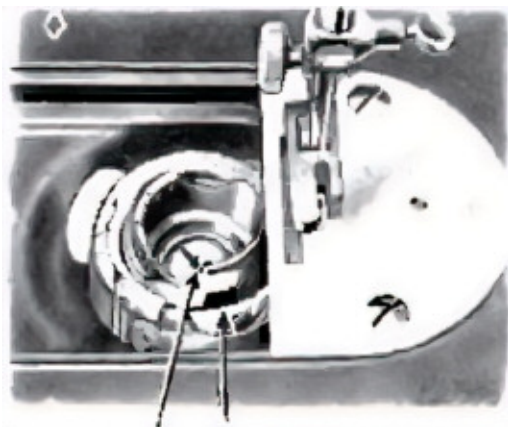
FIG. 65. VIEW OF SEWING HOOK SHOWING OILING POINTS
