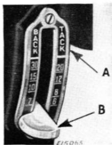
FIG. 16. STITCH REGULATOR
