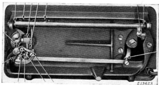
FIG. 18. OILING POINTS AT THE BASE OF MACHINE
