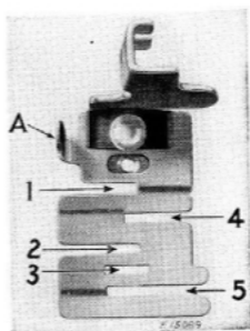
FIG. 41 THE EDGE-STITCHER
