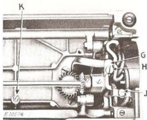
FIG. 5. MOTOR AND SINGERLIGHT LEADS
