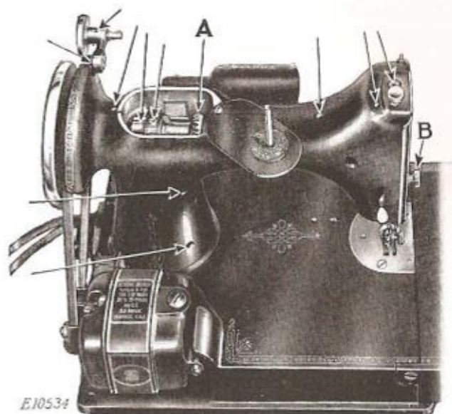
FIG. 34. REAR VIEW, SHOWING OILING POINTS
