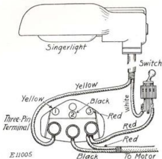
FIG. 2. THREE-PIN TERMINAL AND SINGERLIGHT WIRING DIAGRAM
