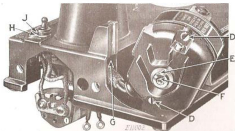
FIG. 14. MOTOR LEADS BEING WITHDRAWN FROM MACHINE
