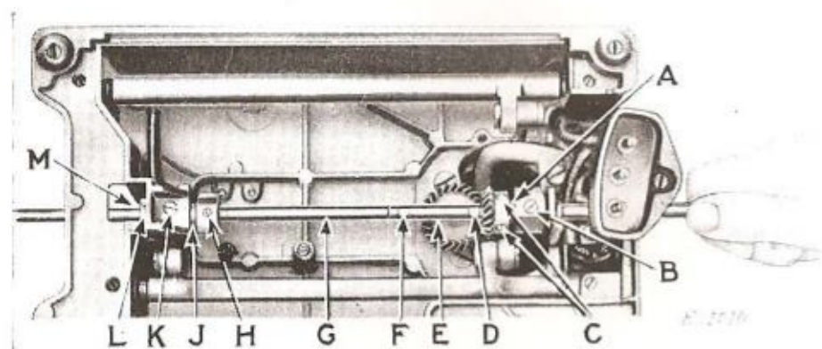
FIG. 25. REPLACING ROTARY SEWING HOOK SHAFT
