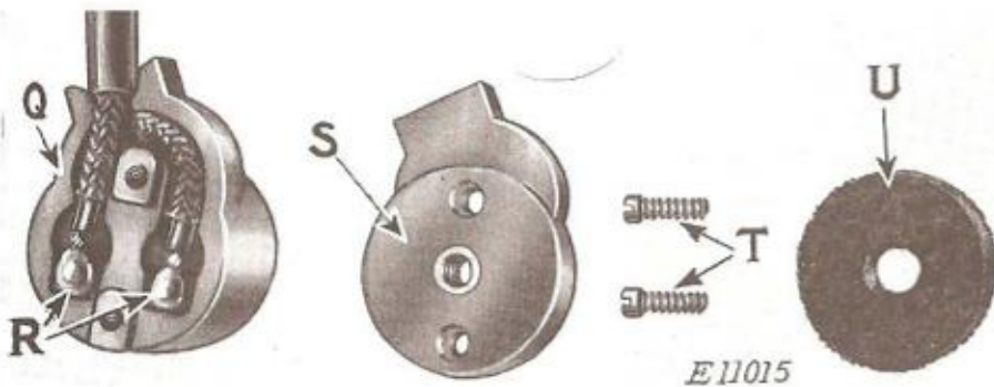
FIG. 7. SINGERLIGHT CONNECTIONS
