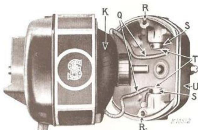
FIG. 16. SERIES 3 MOTOR WITH COMMUTATOR END COVER REMOVED
