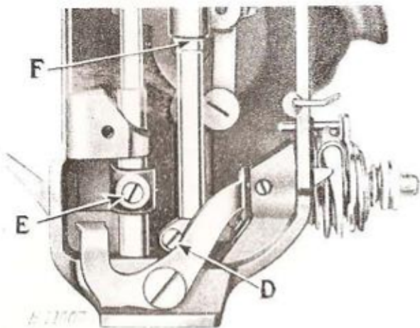
FIG. 21. NEEDLE BAR SET AT CORRECT HEIGHT
