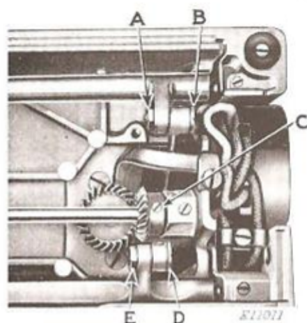
FIG. 29. FEED DOG ADJUSTMENT
