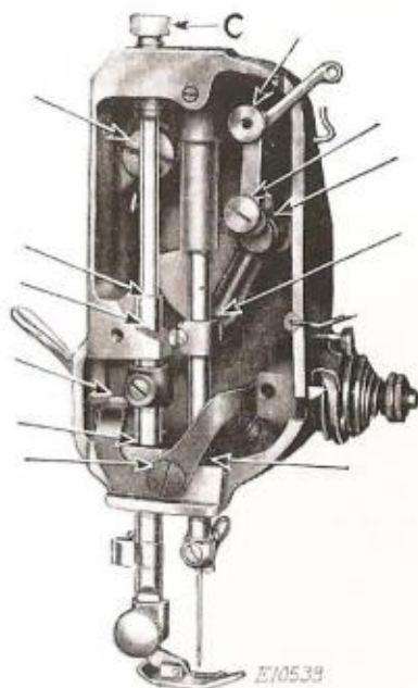
FIG. 35. END VIEW, SHOWING OILING POINTS
