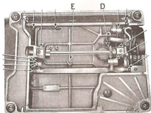
FIG. 36. OILING POINTS IN BASE OF MACHINE
