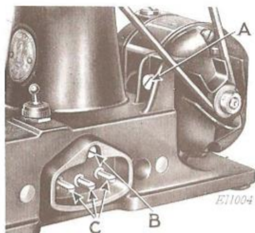
FIG. 13. SHOWING SERIES 3 MOTOR AND THREE-PIN TERMINAL IN PLACE ON MACHINE NO. 221-1
