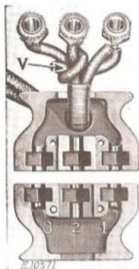
FIG. 9 TERMINAL PLUG (CONNECTIONS REMOVED)
