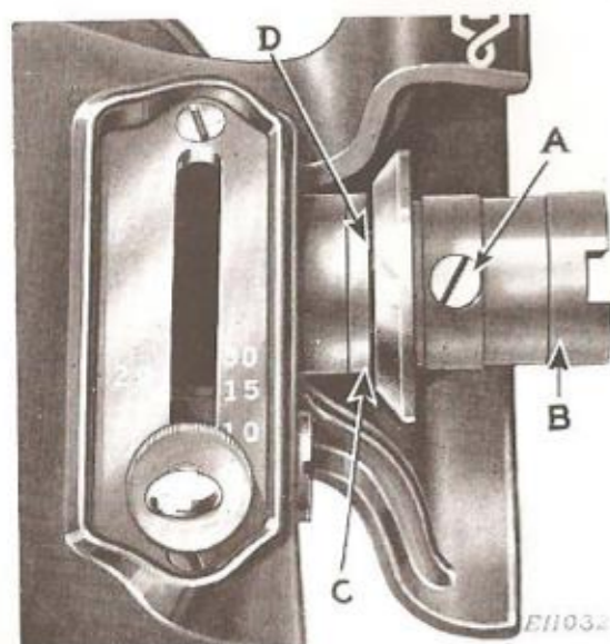
FIG. 33. ADJUSTMENT FOR SHAFT END PLAY
