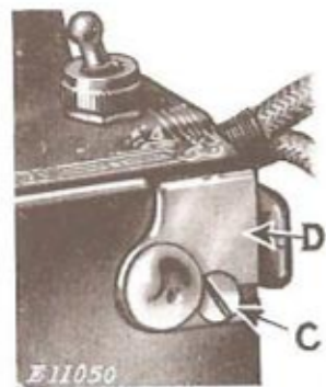
FIG. 31. BOBBIN WINDER TENSION BRACKET
