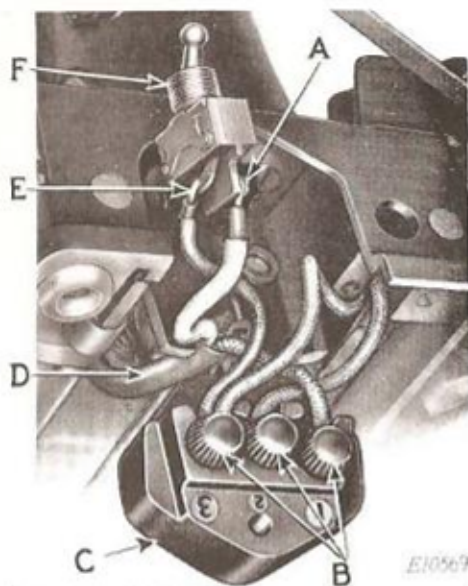
FIG. 4. WIRING, WITH THREE-PIN TERMINAL AND SINGERLIGHT SWITCH DISPLACED
