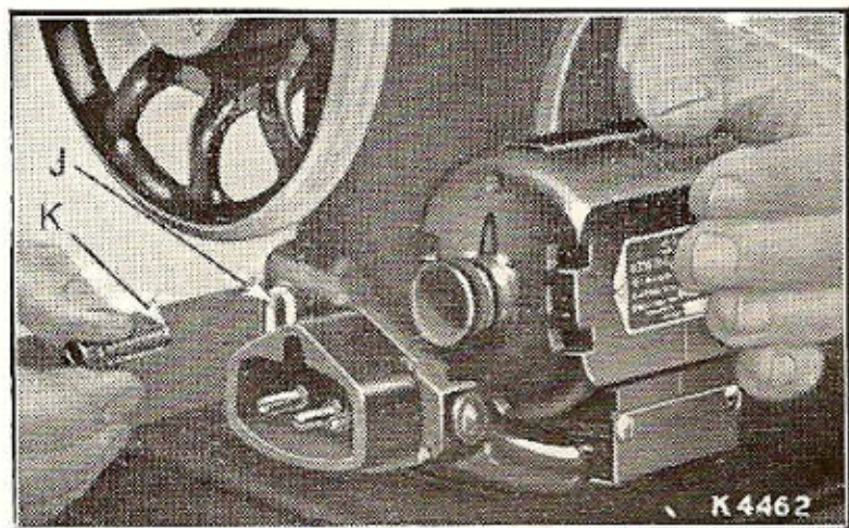
Fig. 3. Placing the Motor in Position.
