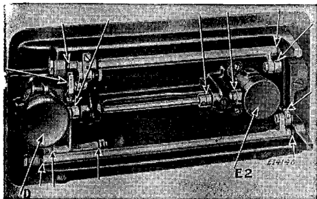
Fig. 30. Oiling Points in Bed of Machine.
