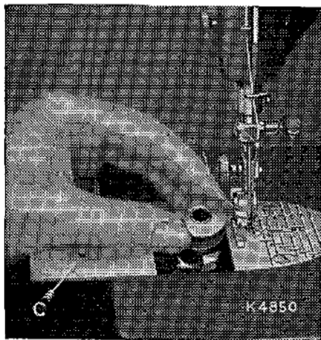
Fig. 11. Removing the Bobbin.
