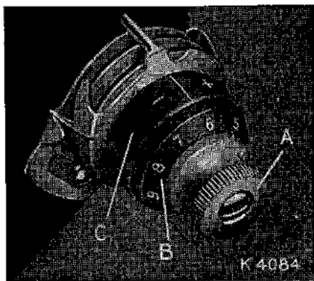
Fig. 25. To Regulate Needle Thread Tension.
