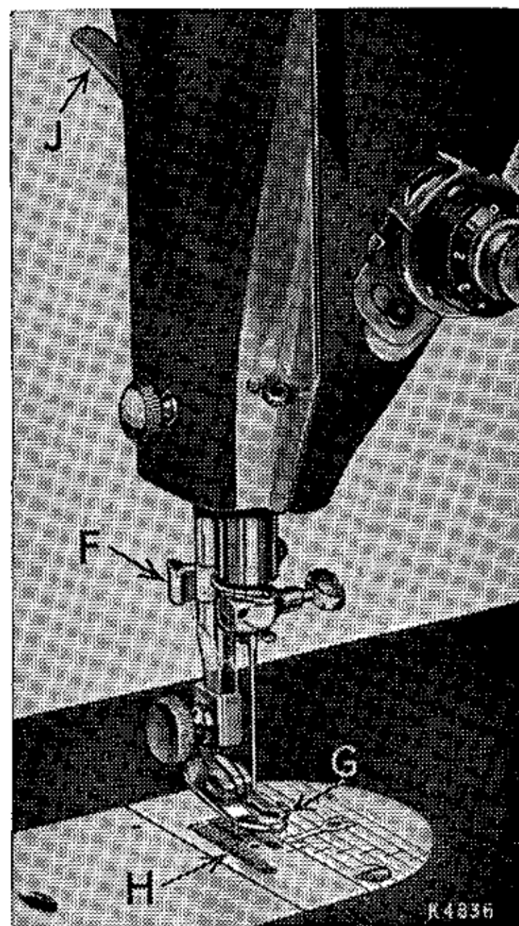
Fig. 5. Front view of machine.
