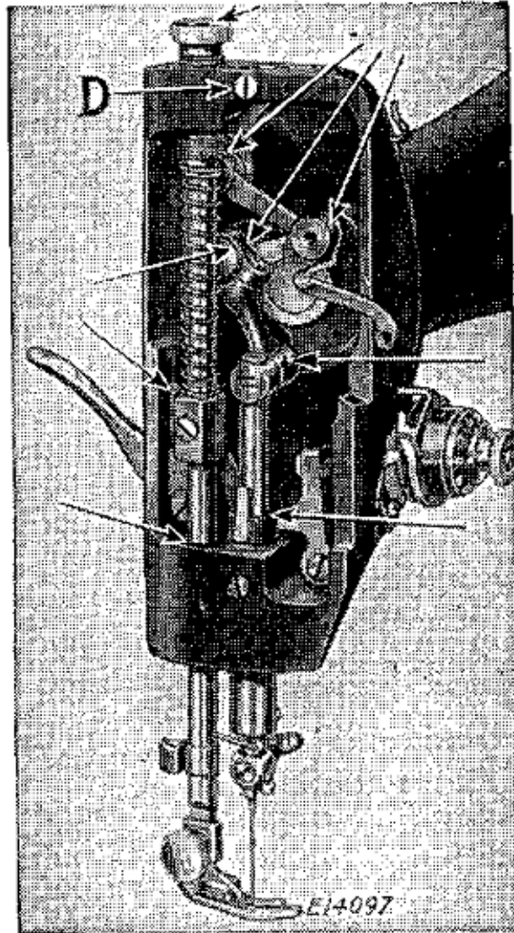
Fig. 28. Face Plate Removed, Showing Oiling Points.
