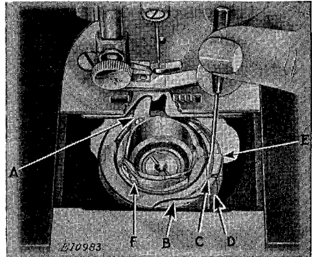
Fig. 32. Bobbin Case in Position. (Throat Plate broken away to show correct location of Finger A).
