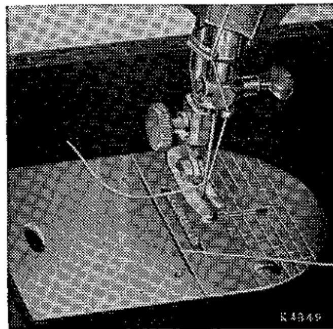
Fig. 17. Under Threading Completed.
