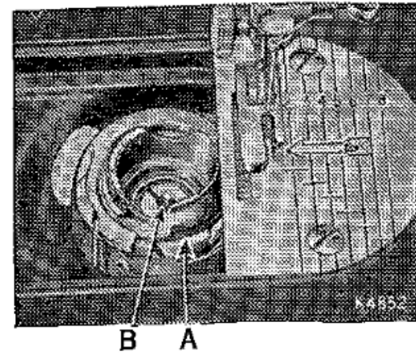
Fig. 29. Oiling the Sewing Hook.
