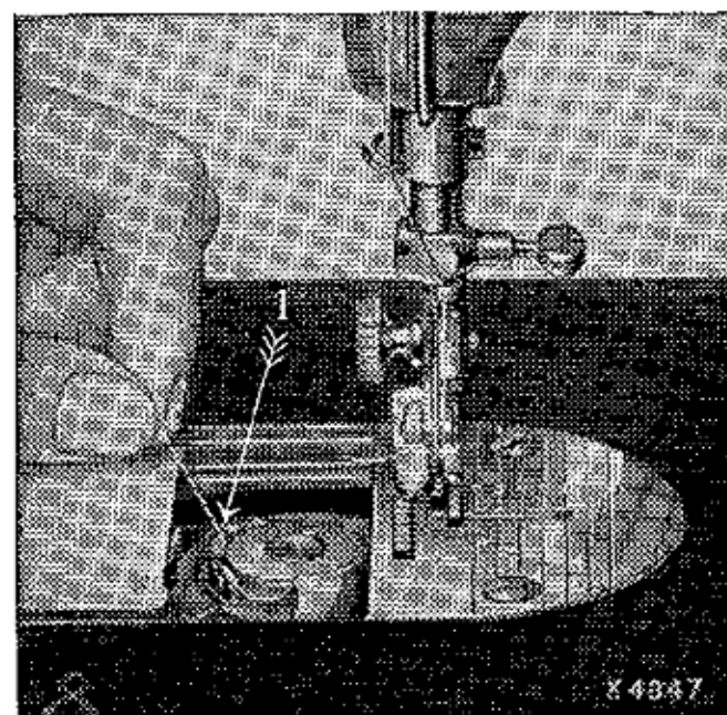
Fig. 15. Threading the Bobbin Case.
