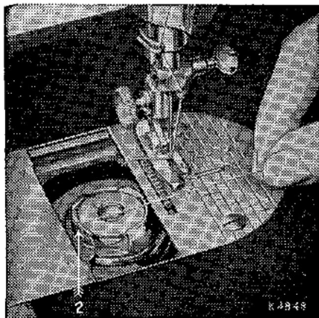
Fig. 16. Bobbin Case Threaded.
