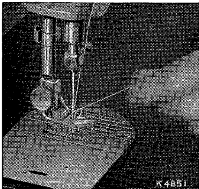
Fig. 18. Drawing Up the Under Thread.
