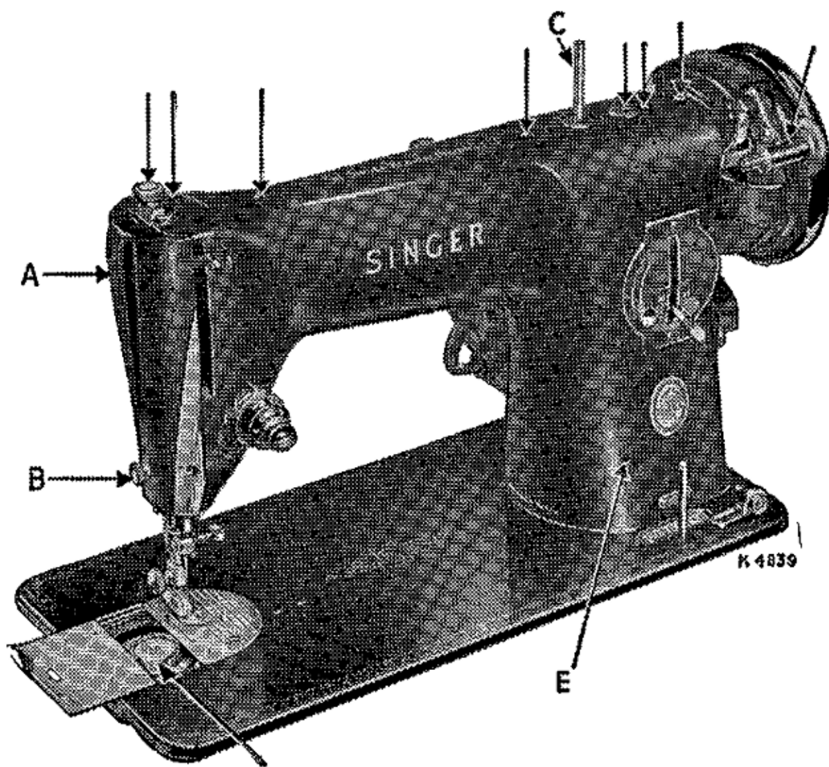
Fig. 27. Front View, Showing Oiling Points.
