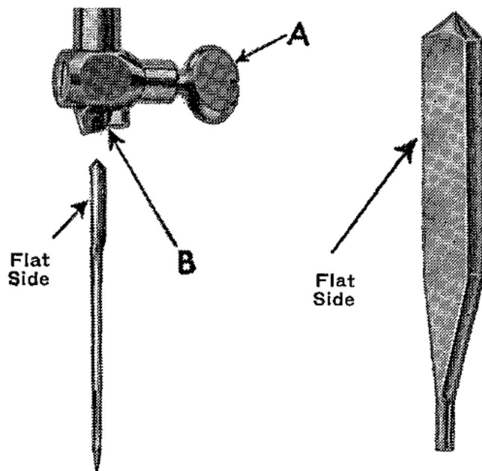
Fig. 9. Setting the Needle.
