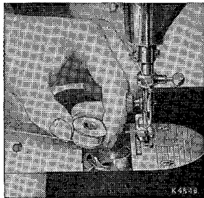
Fig. 14. Replacing the Bobbin.
