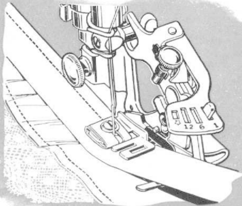
Fig. 66. Correct Positions for Materials
