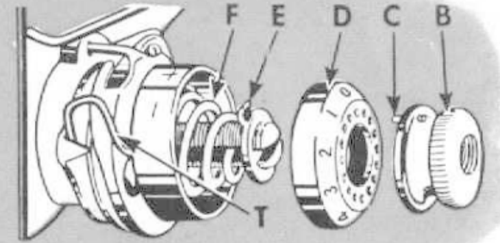
Fig. 27. Reassembling Needle Thread Tension
