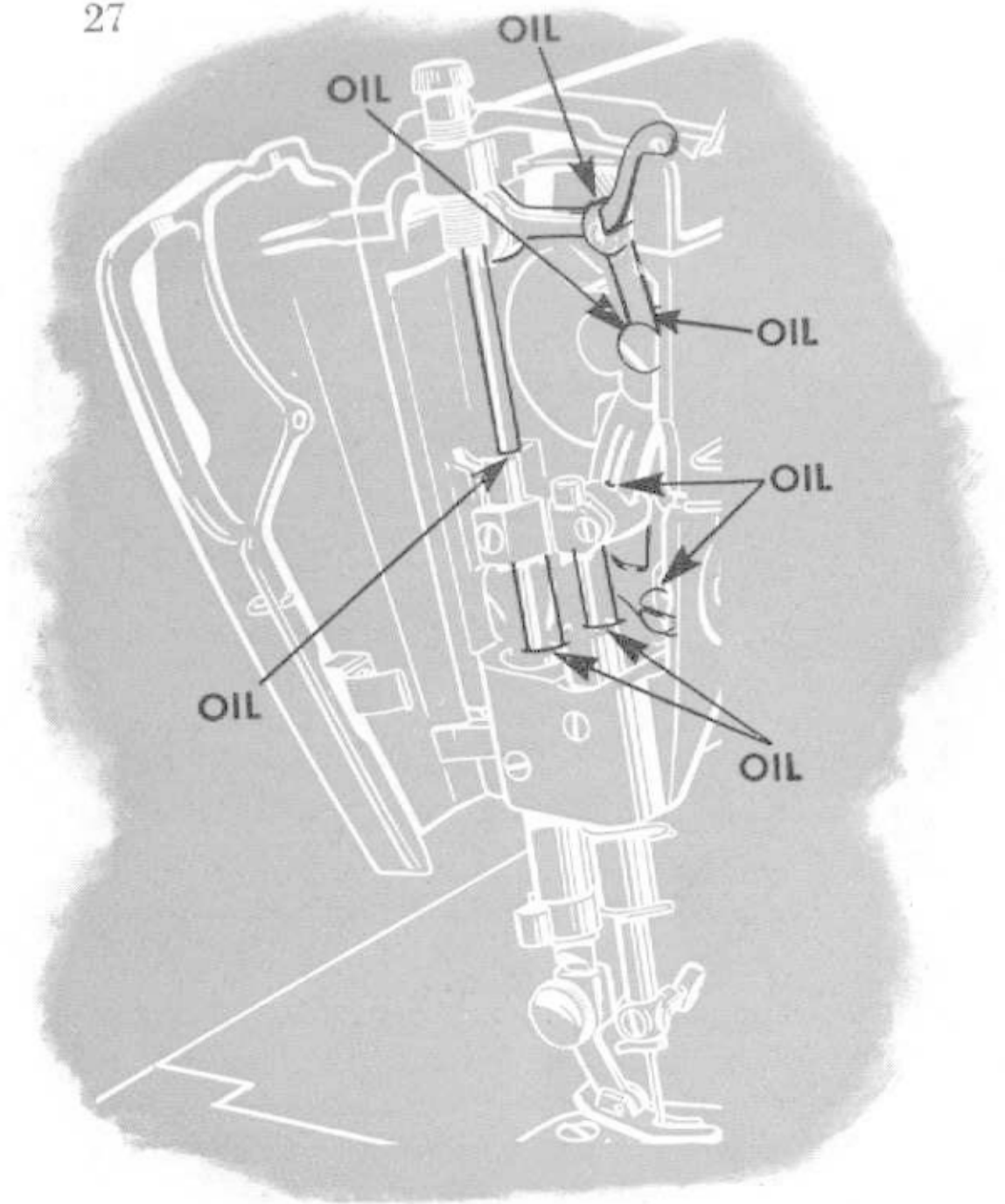
Fig. 31. Face Plate Opened Showing Oiling Points
