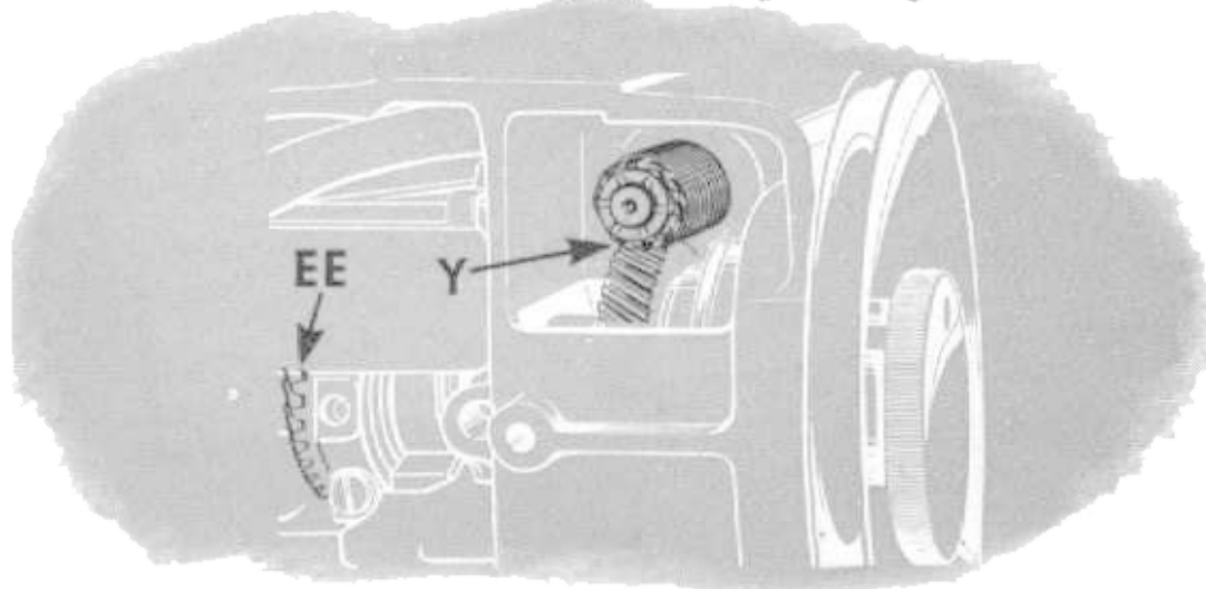
Fig. 30. Lubricating Points for Spiral Gears in Top of Machine
