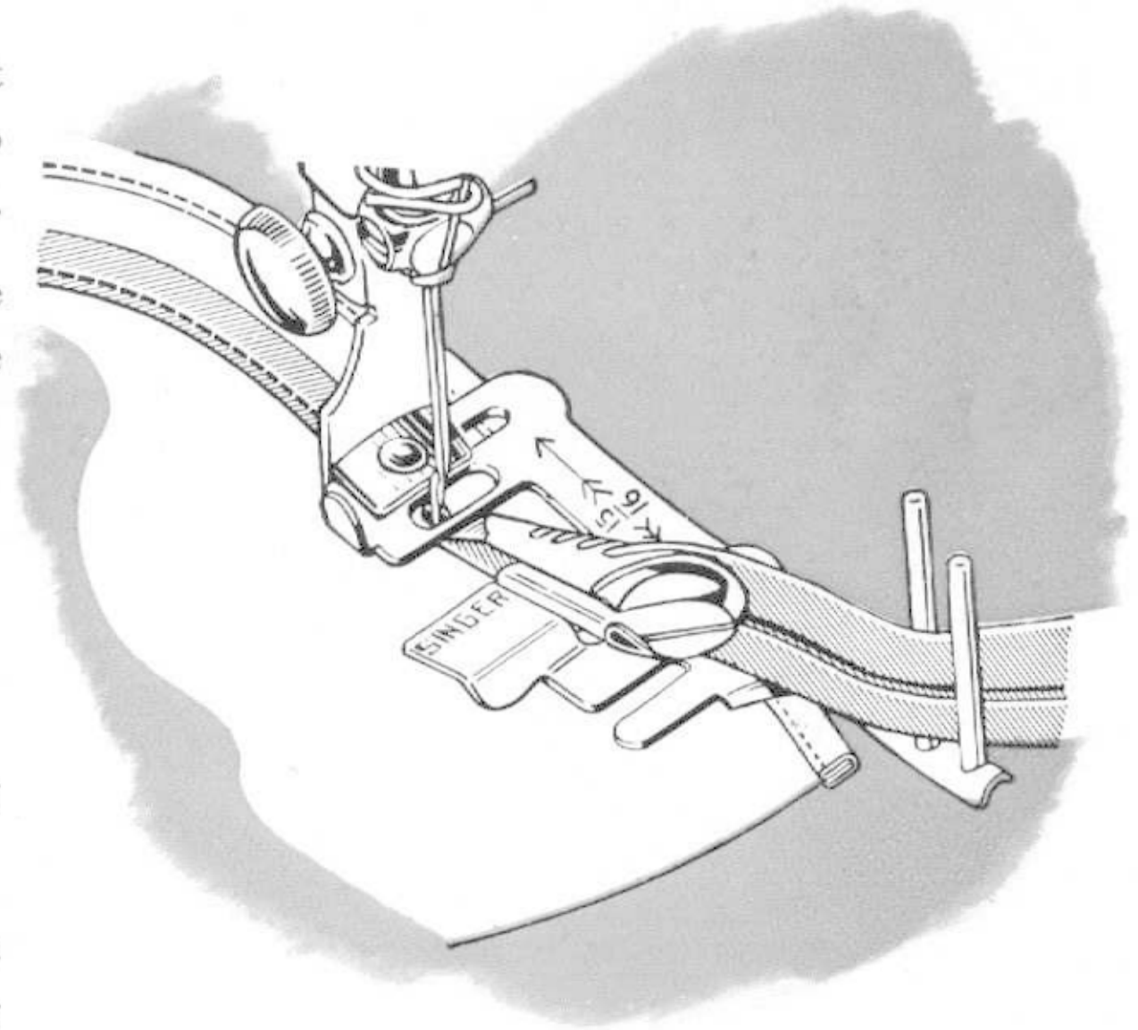
Fig. 51. Applying a French Fold
