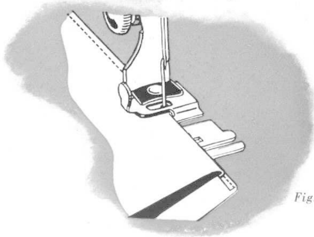
Fig. 57. Making a Wide Hem
