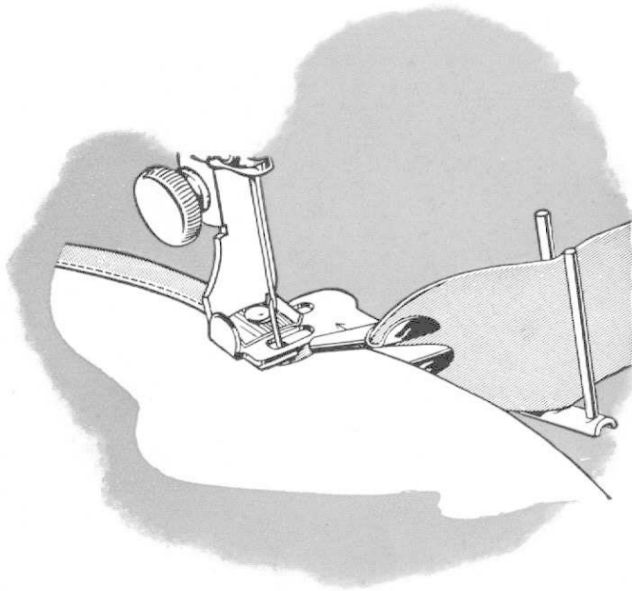
Fig. 50. Binding on Outside Curve
