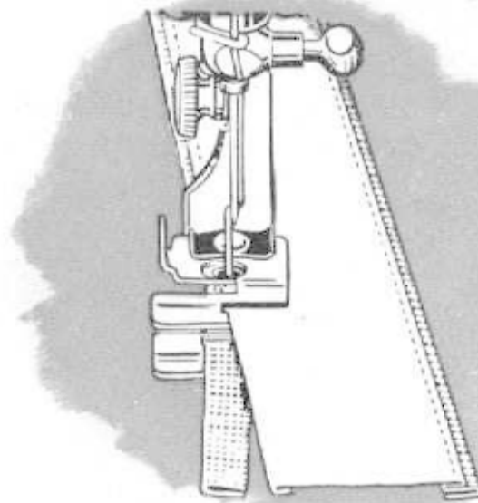
Fig. 54. Setting in Lace Insertion
