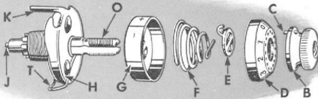
Fig. 25. Needle Thread Tension Disassembled
