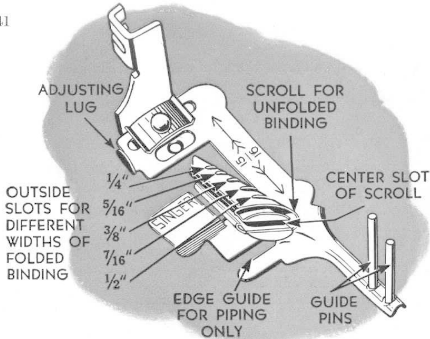
Fig. 45. Multi-Slotted Binder 160624
