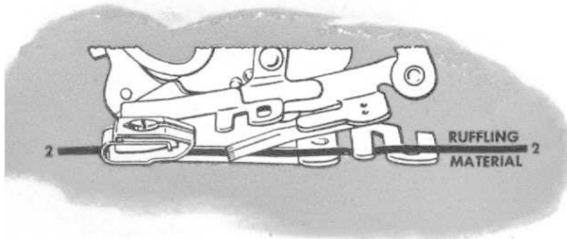
Fig. 71. Correct Position for Material
