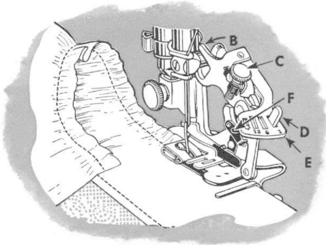
Fig. 62. Gathering with Ruffler
