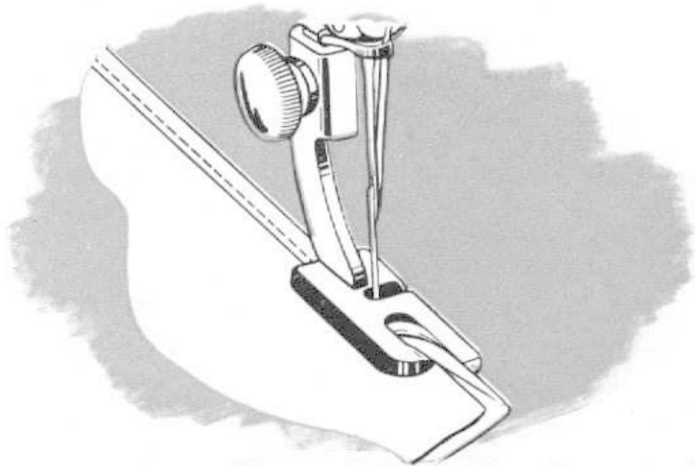
Fig. 38. Making a Hemmed Seam (First Operation)
