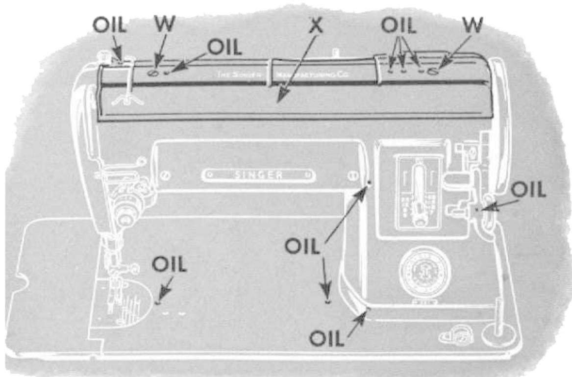
Fig. 29. Front View, Showing Oiling Points
