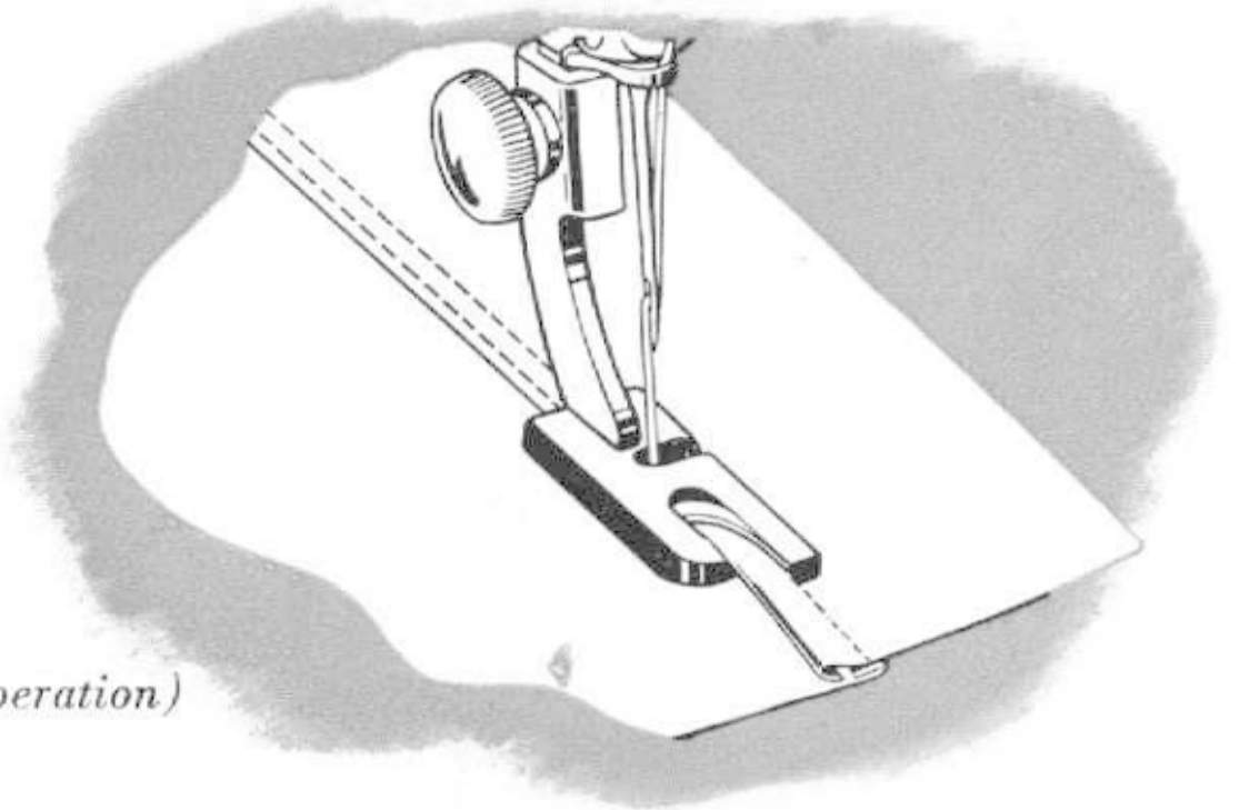
Fig. 40. Making a Felled Seam (First Operation)
