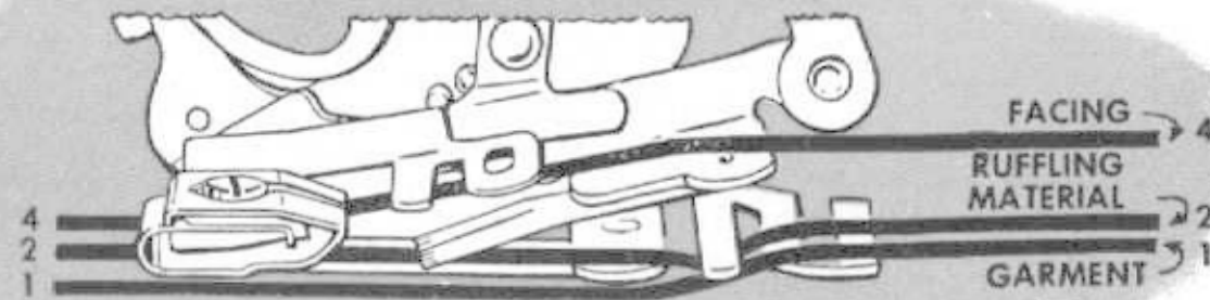
Fig. 66. Correct Positions for Materials
