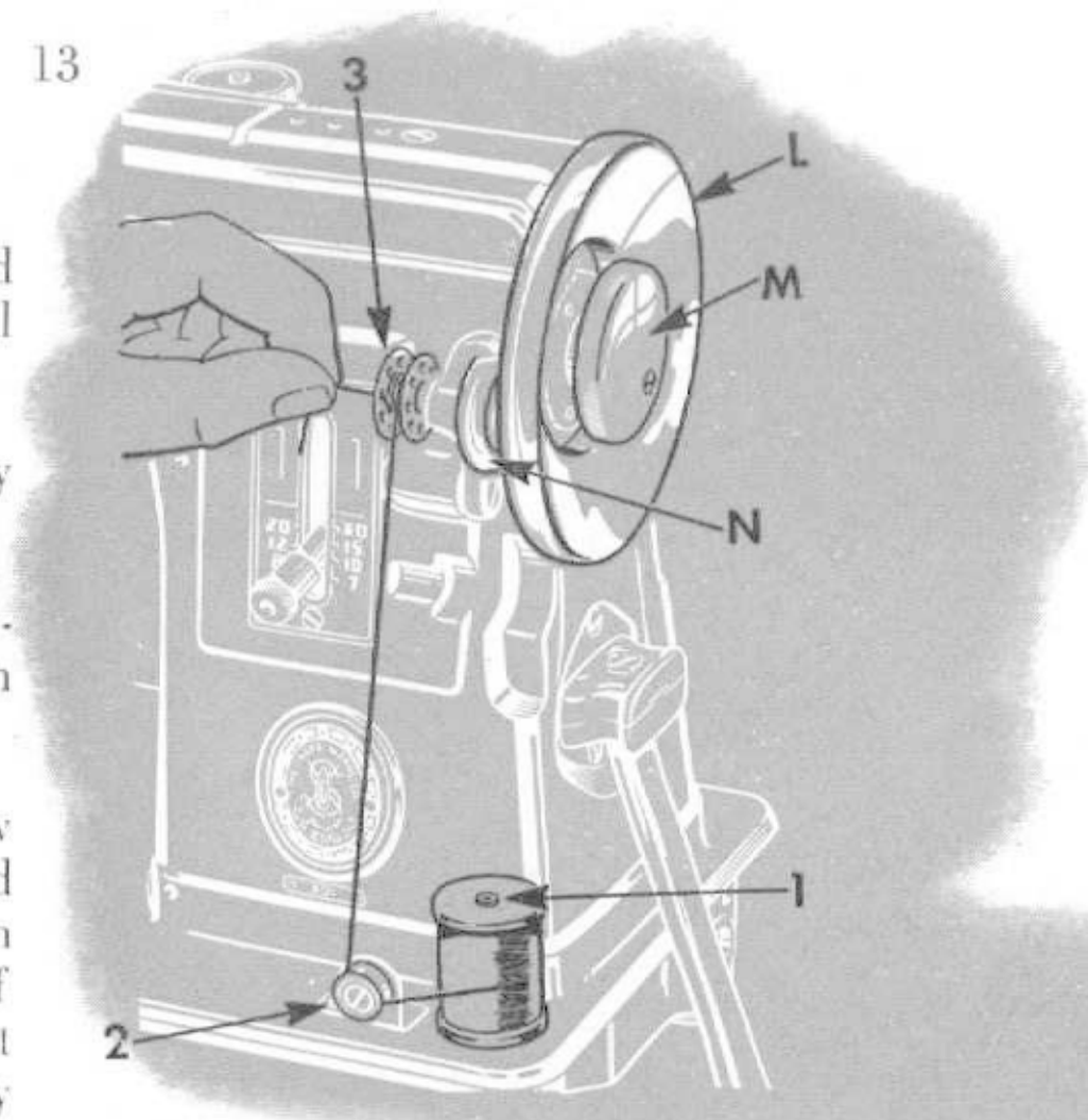
Fig. 9. Winding the Bobbin
