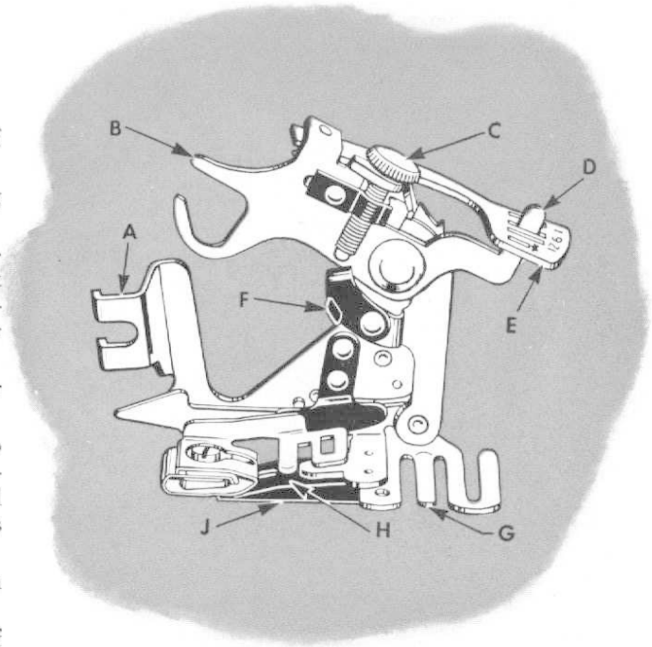
Fig. 61. Principal Parts of Ruffler
