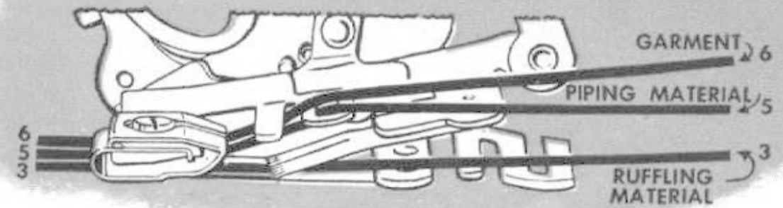
Fig. 68. Correct Positions for Materials
