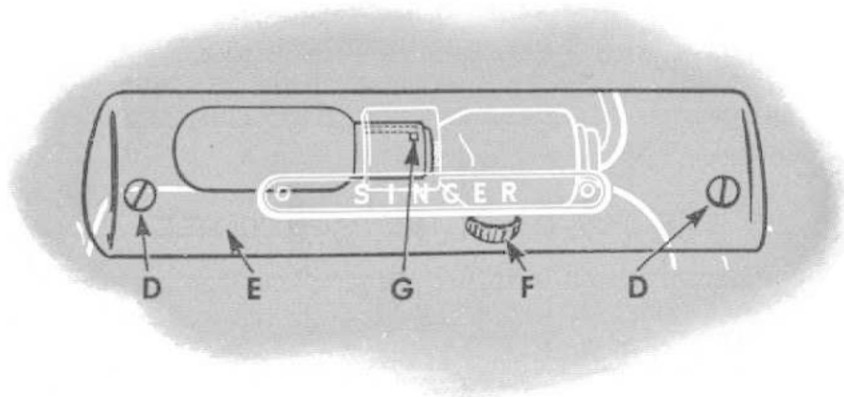
Fig. 4. Replacing the Bulb
